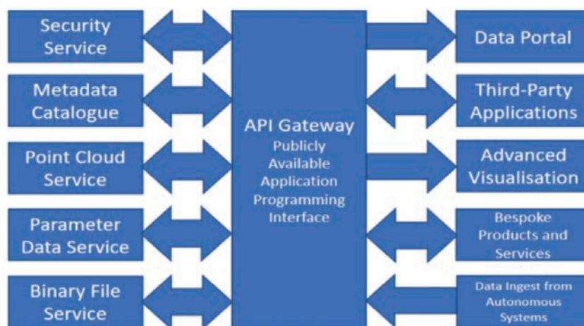
Fig. 1 - An overview of the iMarDIS architecture showing the 'back end' microservices to the left of the Application Programming Interface and the applications domain on the right handside. The applications domain is where advanced service capability can be implemented either by iMarDIS or third party developers.
