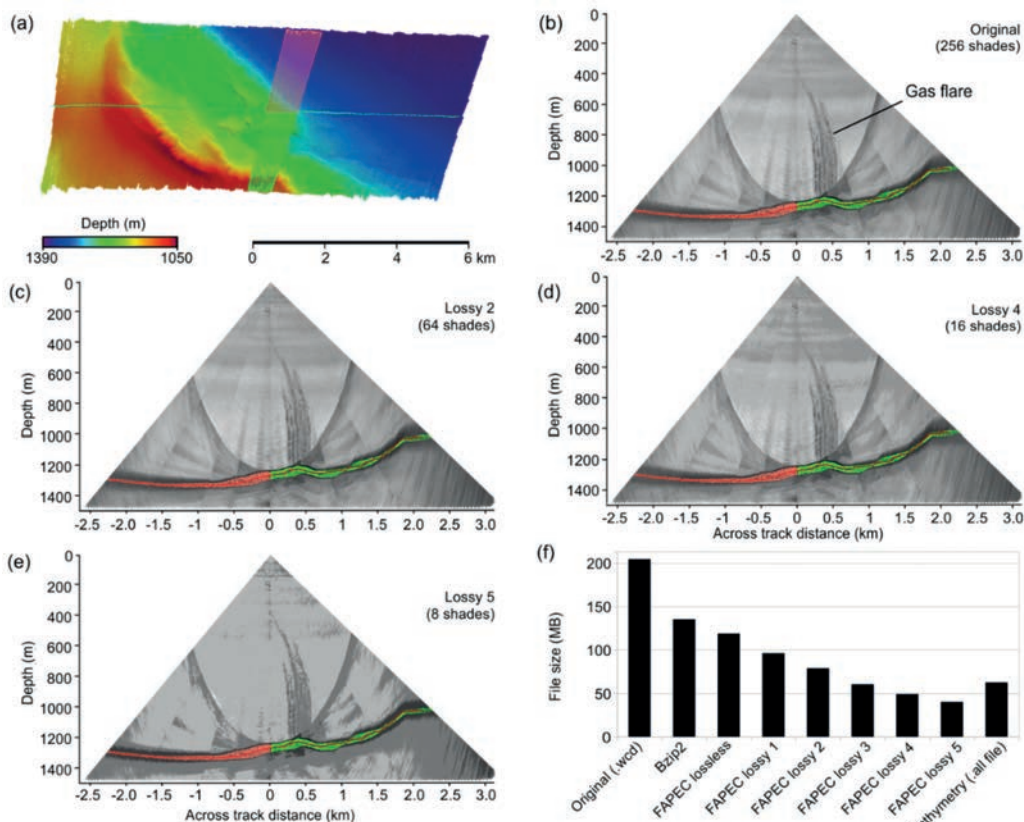
Fig. 2 - EM302 scene (a) showing the original water column (b) and that obtained with different levels of FAPEC lossy compression (c), (d) and (e). Panel (f) shows the corresponding file sizes, including bzip2 compression for comparison. Features in the water column such as gas seeps can still be detected even with low-quality compression levels. Actually, such levels seem to provide an even clearer evidence of the gas-related features.
