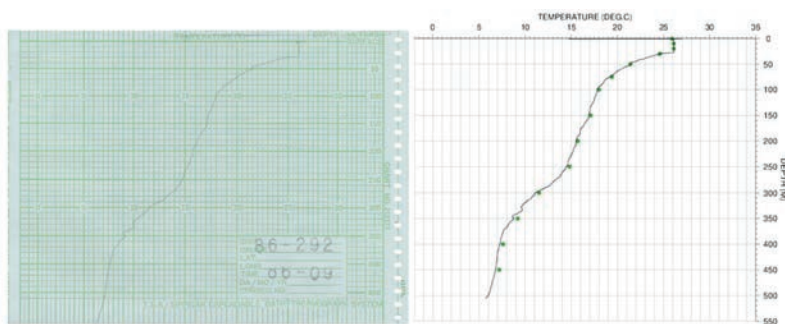
Fig. 1 - Examples of XBT strip chart by R/V Ryofu-Maru of Japan Meteorological Agency (left panel), and traced temperature profile (black line in right panel) and visual reading temperature at the standard depths (green circle in right panel).
