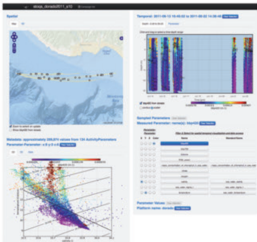
Fig. 1 - STOQS web user interface.
