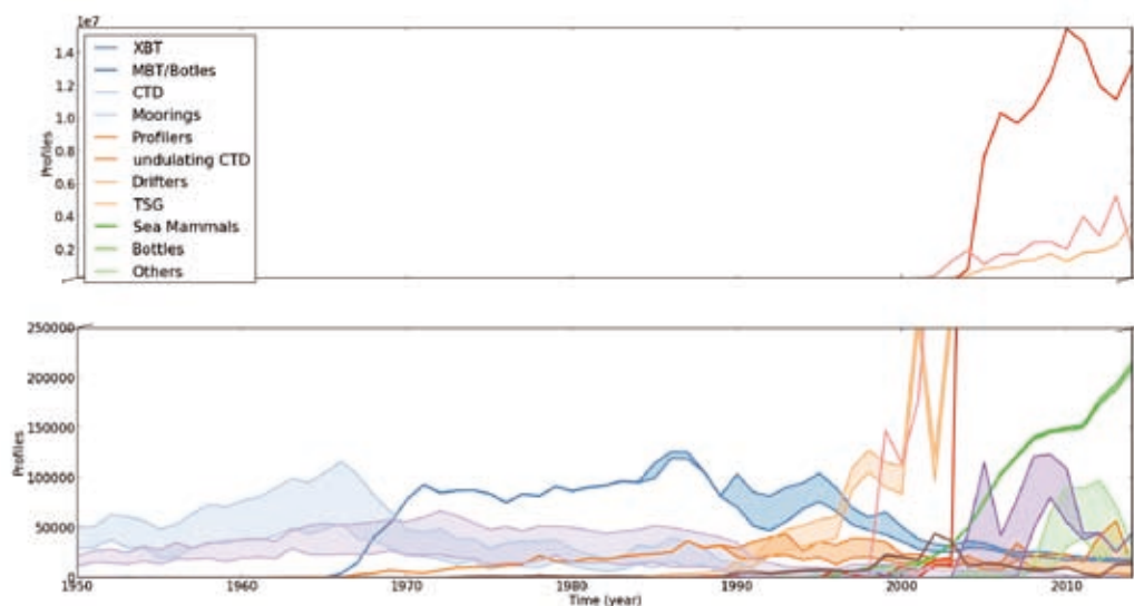
Fig. 1 - Yearly number of CORA profiles for various instrument types. For each instrument types, the lower line refers to CORA4.2 (released on april 2016) dataset and the upper line refers to the estimated number of profiles for the CORA4.3 dataset (to be released on april 2017).
