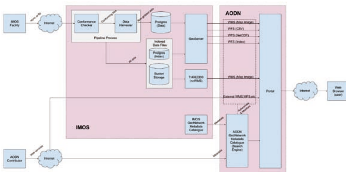
Fig. 1 - IMOS infrastructure at AWS.
