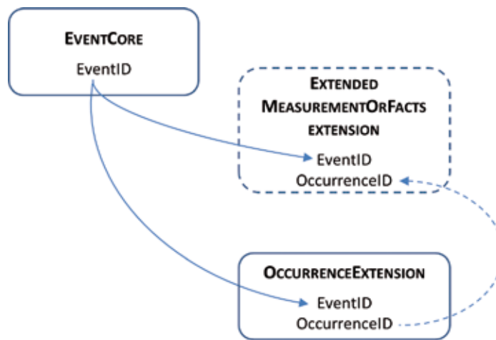
Fig. 1 - Schematic representation of the chosen option. The characteristic IPT star scheme is maintained. An additional linkage for the biological data is added, more specifically between the Occurrence extension and the newly adopted Extended MeasurementOrFacts extension (eMOF).
