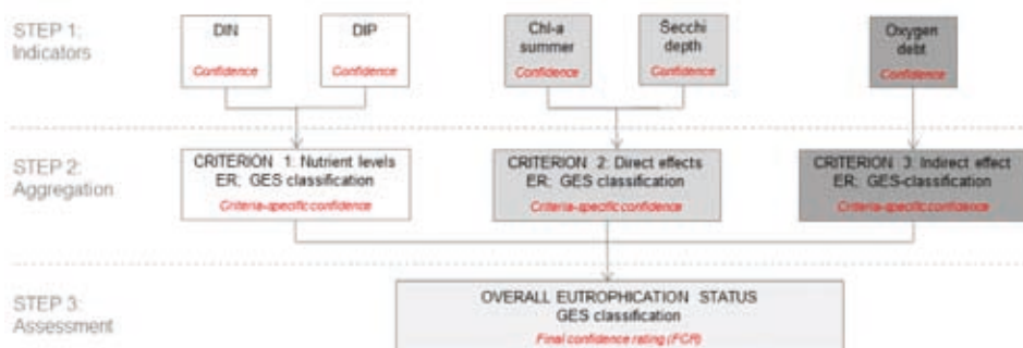
Fig. 2 - Schematic visualization of how the eutrophication status assessment is produced in open-sea assessment units using HEAT 3.0 and the core indicators.
