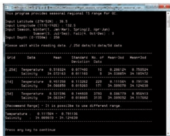
Fig. 1 - Program to calculate seasonal regional QC range.
